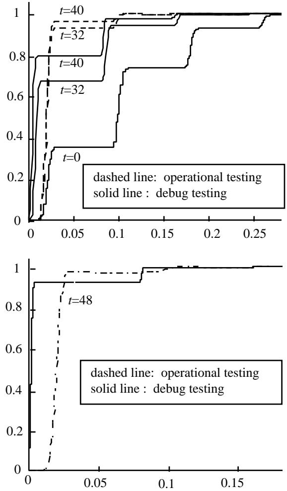
Figure 5. Cumulative distribution functions of the failure rate \lambda , before testing and then at three stages in the testing: before, at, and (lower figure) after the crossover point of the mean values (cf. Fig 4).
